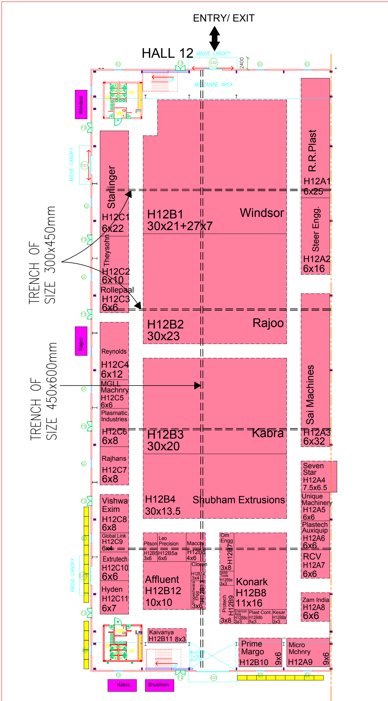
KEY PLAN
